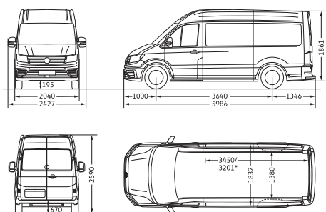
Crafter 35 Van MWB high roof
